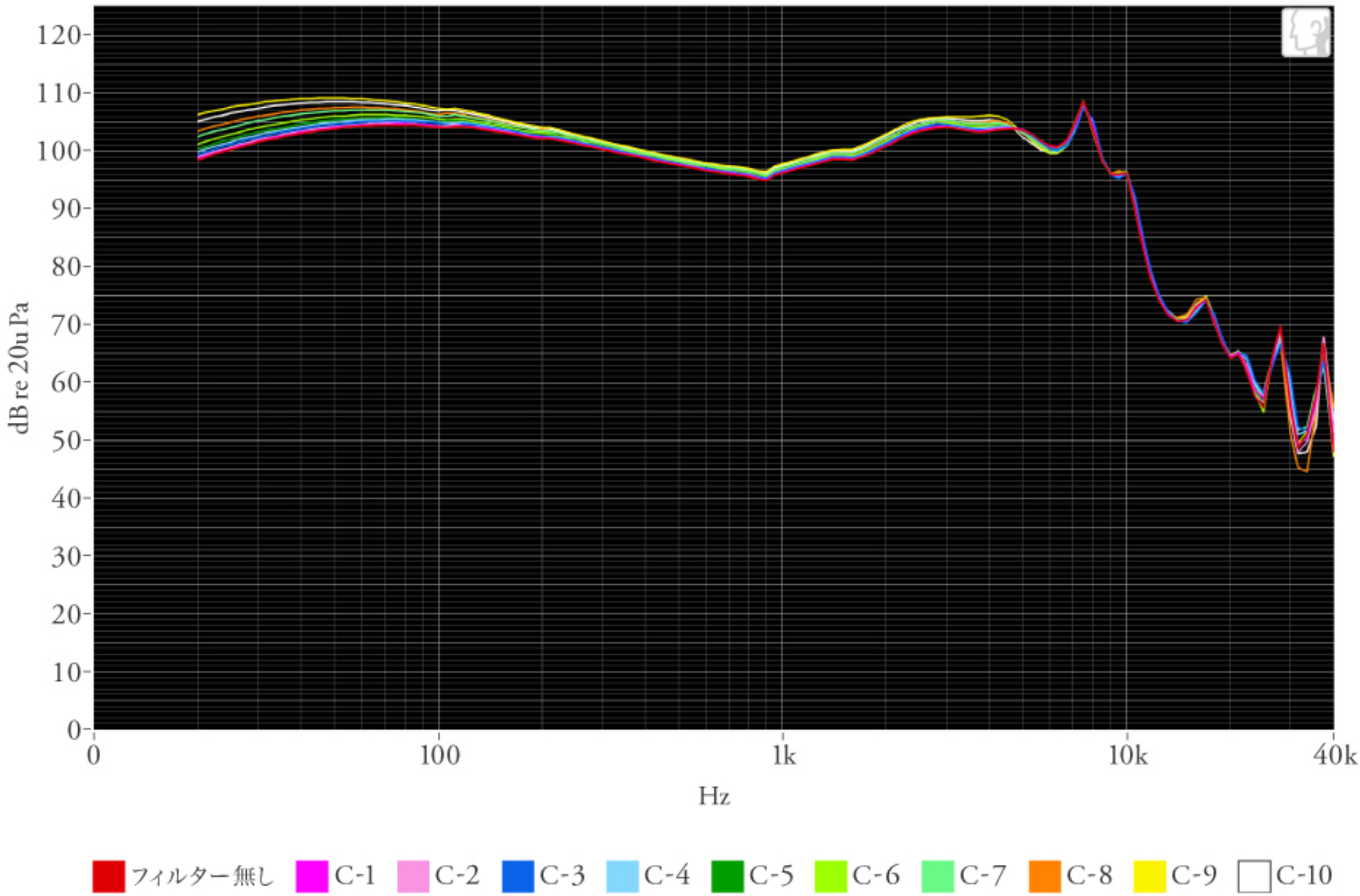
— Filter C Frequency Response Graph —
